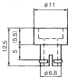
4mmねじ用ブッシュ Bushing for 4mm screw
